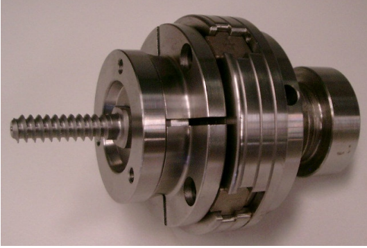
Chuck Screw Faceplate mounted on chuck
